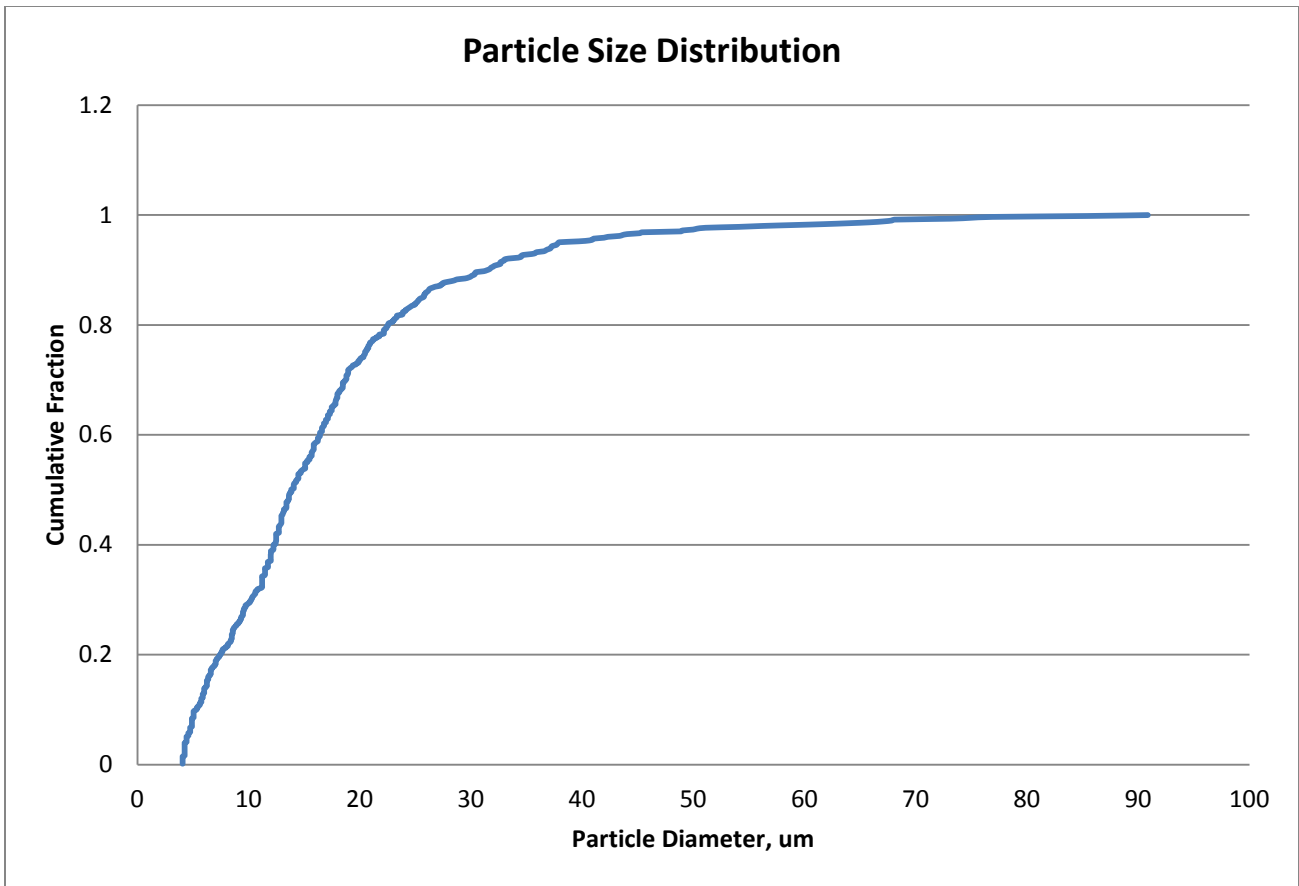
Figure 5: Particle size distribution of Phenolphthalein.
