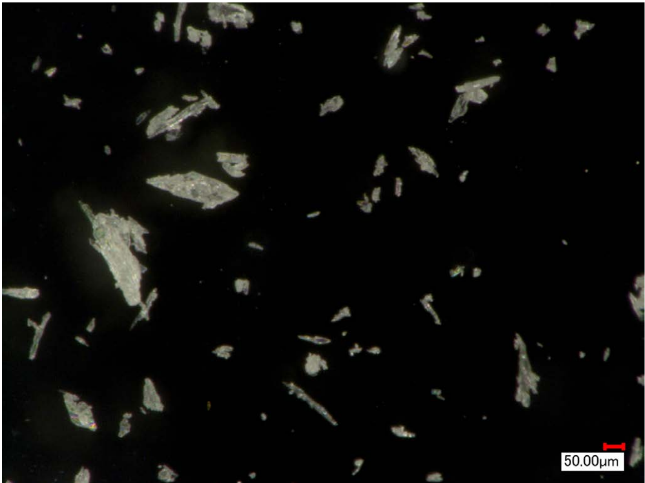
Figure 4: Photomicrograph of Ground Dimethyl Terephthalate crystals.
