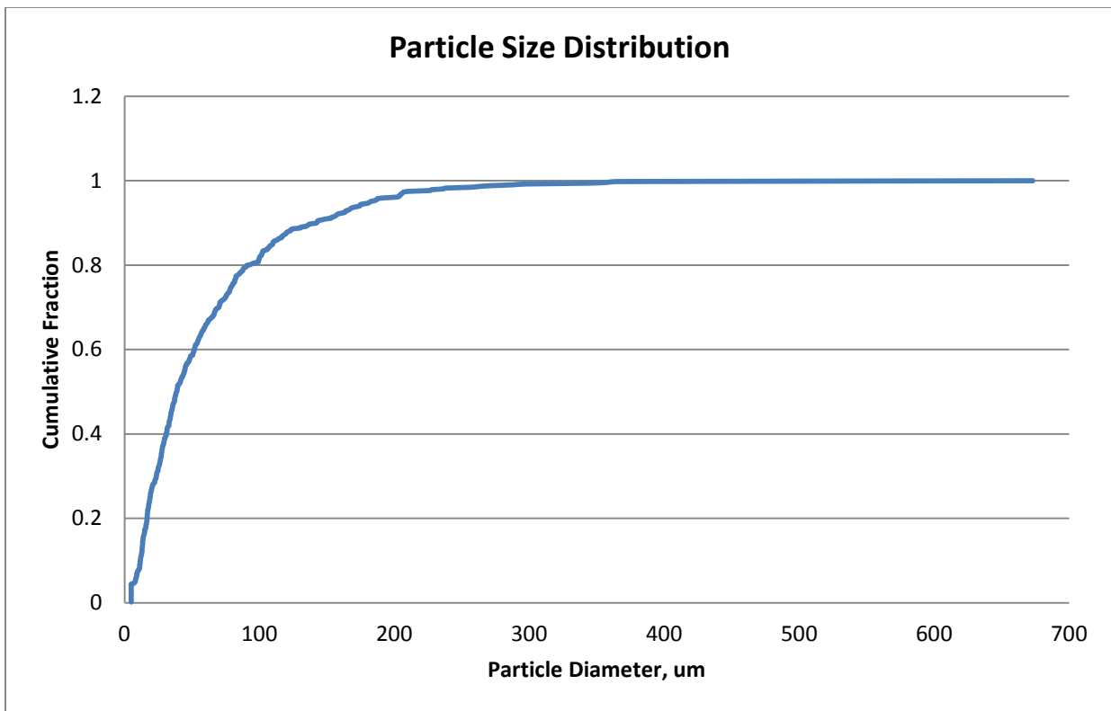
Figure 5: Particle size distribution of Ground Dimethyl Terephthalate crystals.
